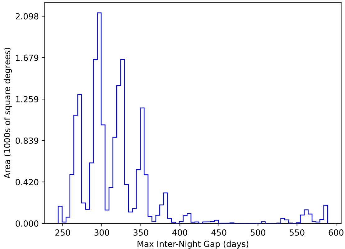
ddf_acor_sf10_lsf15_lsr20_v3.4_10yrs WFD y band: Max Inter-Night Gap
