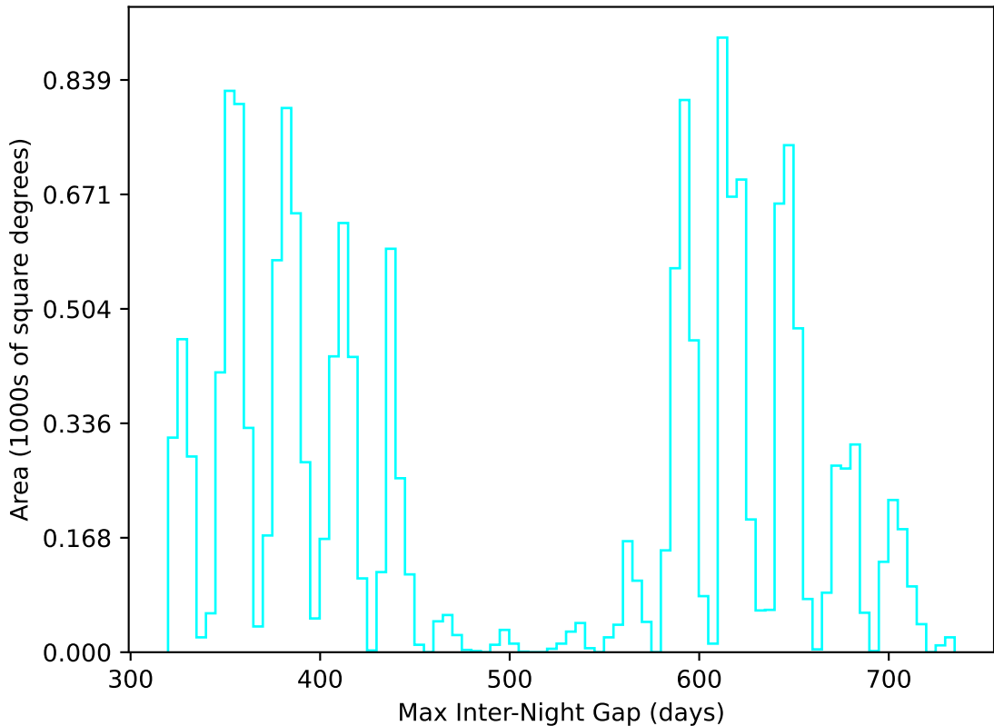
ddf_acor_sf10_lsf15_lsr20_v3.4_10yrs WFD u band: Max Inter-Night Gap
