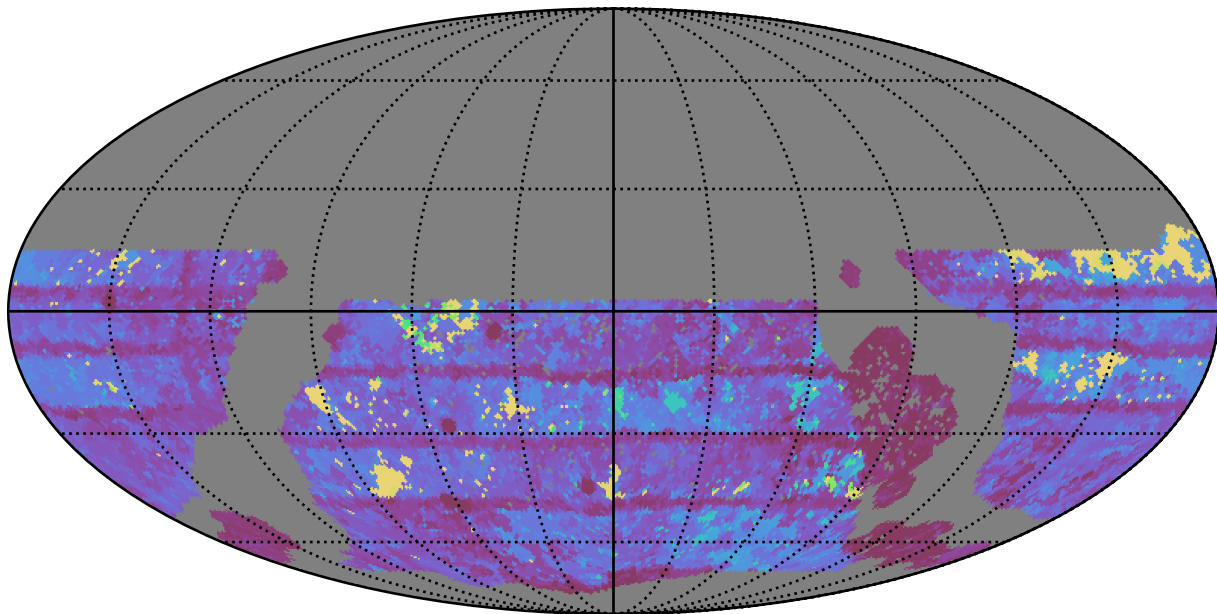
ddf_acor_sf10_lsf15_lsr20_v3.4_10yrs WFD r band: Max Inter-Night Gap
