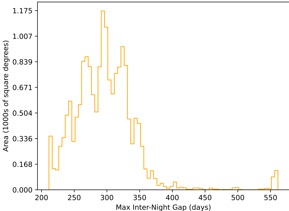
ddf_acor_sf10_lsf15_lsr20_v3.4_10yrs WFD r band: Max Inter-Night Gap
