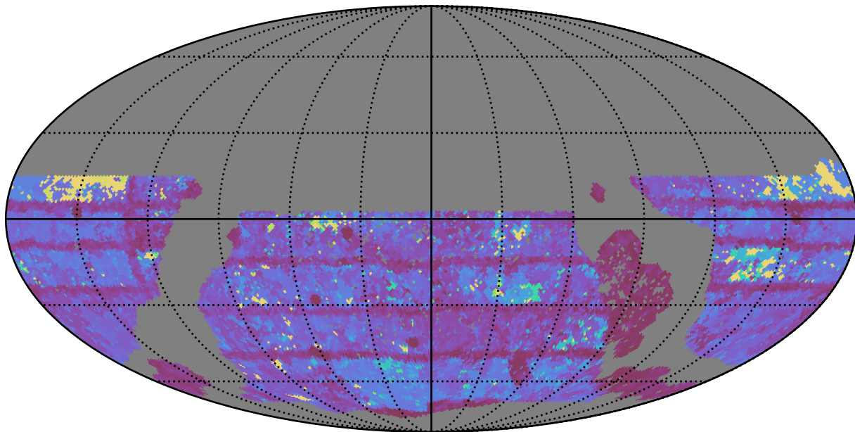
ddf_acor_sf10_lsf15_lsr20_v3.4_10yrs WFD i band: Max Inter-Night Gap
