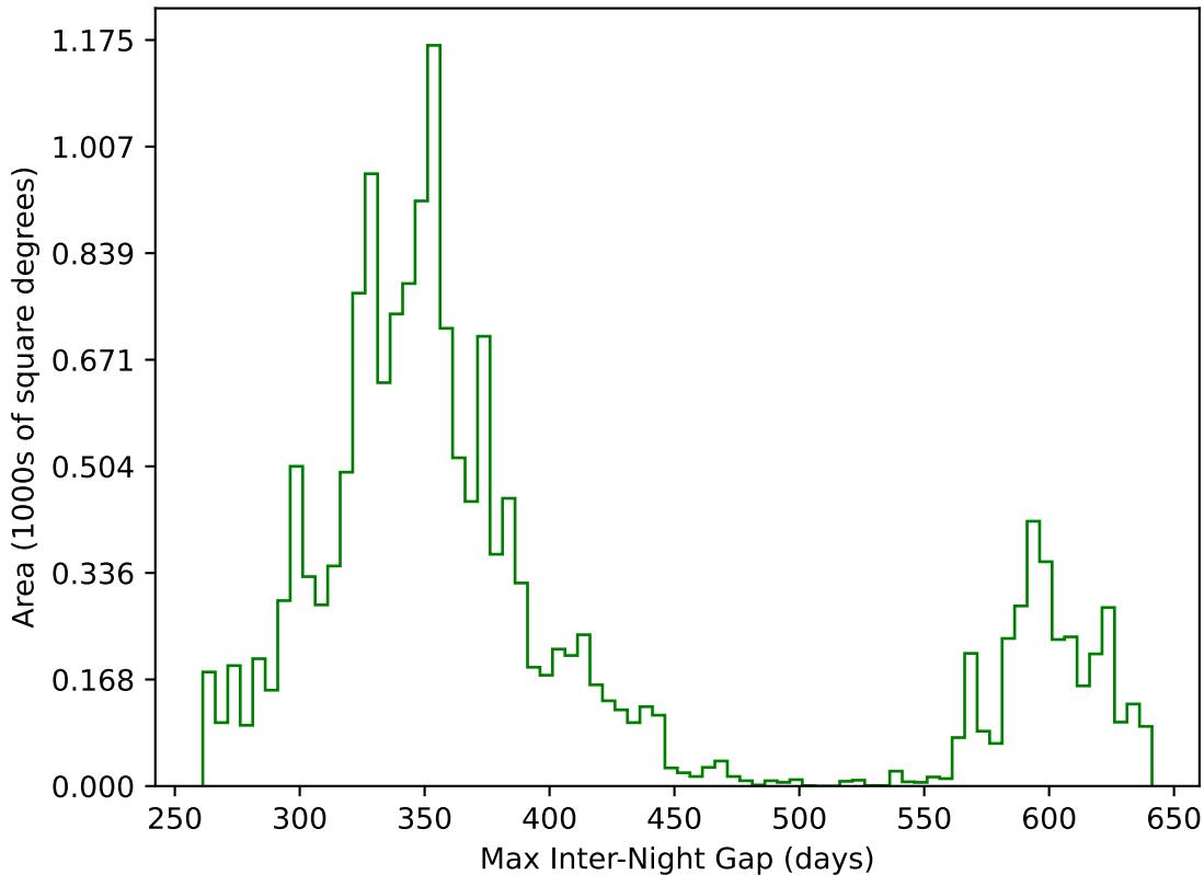
ddf_acor_sf10_lsf15_lsr20_v3.4_10yrs WFD g band: Max Inter-Night Gap
