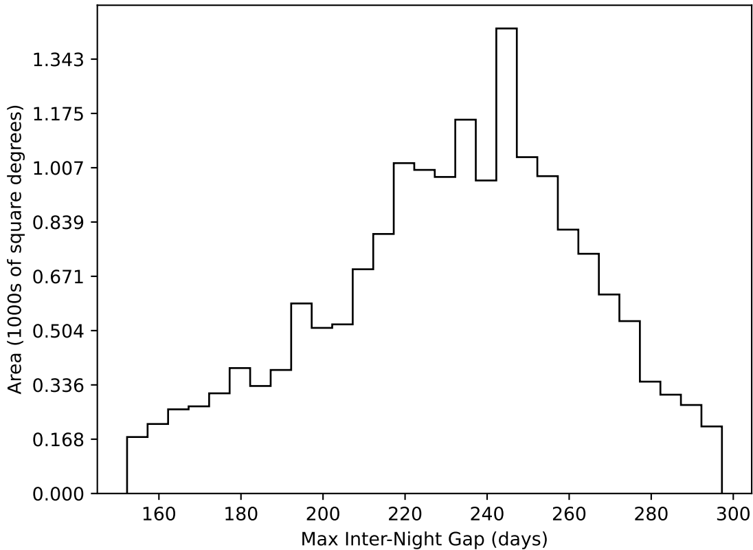
ddf_acor_sf10_lsf15_lsr20_v3.4_10yrs WFD all bands: Max Inter-Night Gap
