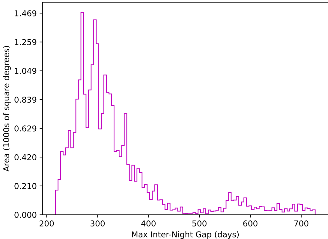
ddf_acor_sf10_lsf15_lsr20_v3.4_10yrs All sky z band: Max Inter-Night Gap
