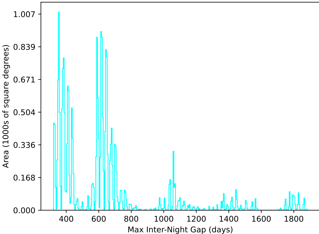
ddf_acor_sf10_lsf15_lsr20_v3.4_10yrs All sky u band: Max Inter-Night Gap
