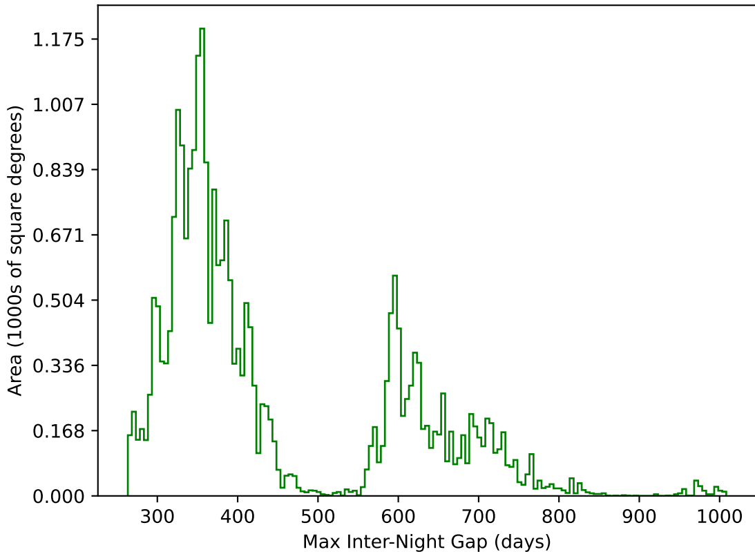
ddf_acor_sf10_ls15_lsr20_v3.4_10yrs All sky g band: Max Inter-Night Gap
