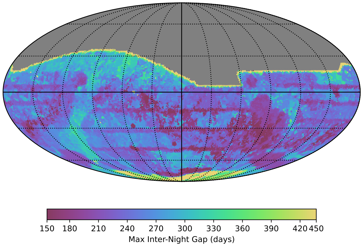
ddf_acor_sf10_lsf15_lsr20_v3.4_10yrs All sky all bands: Max Inter-Night Gap
