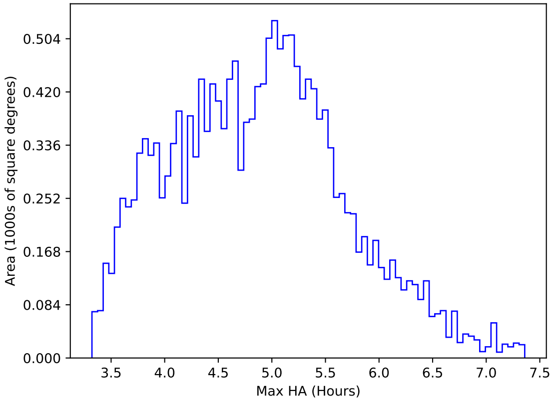
ddf_acor_sf10_lsf15_lsr20_v3.4_10yrs WFD z band: Max HA
