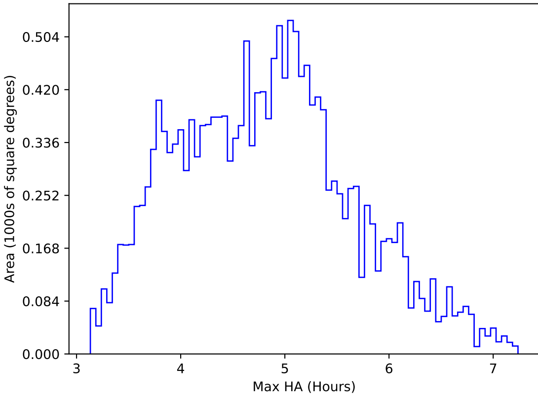
ddf_acor_sf10_lsf15_lsr20_v3.4_10yrs WFD i band: Max HA
