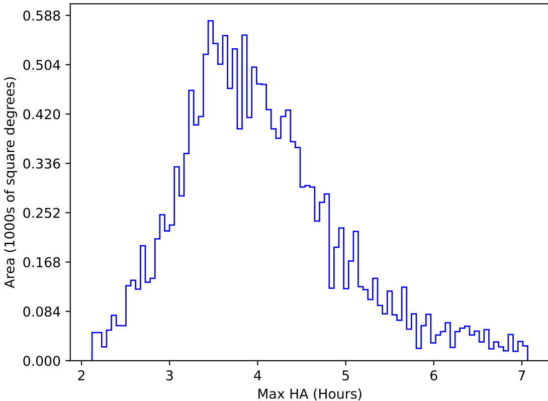
ddf_acor_sf10_lsf15_lsr20_v3.4_10yrs WFD g band: Max HA
