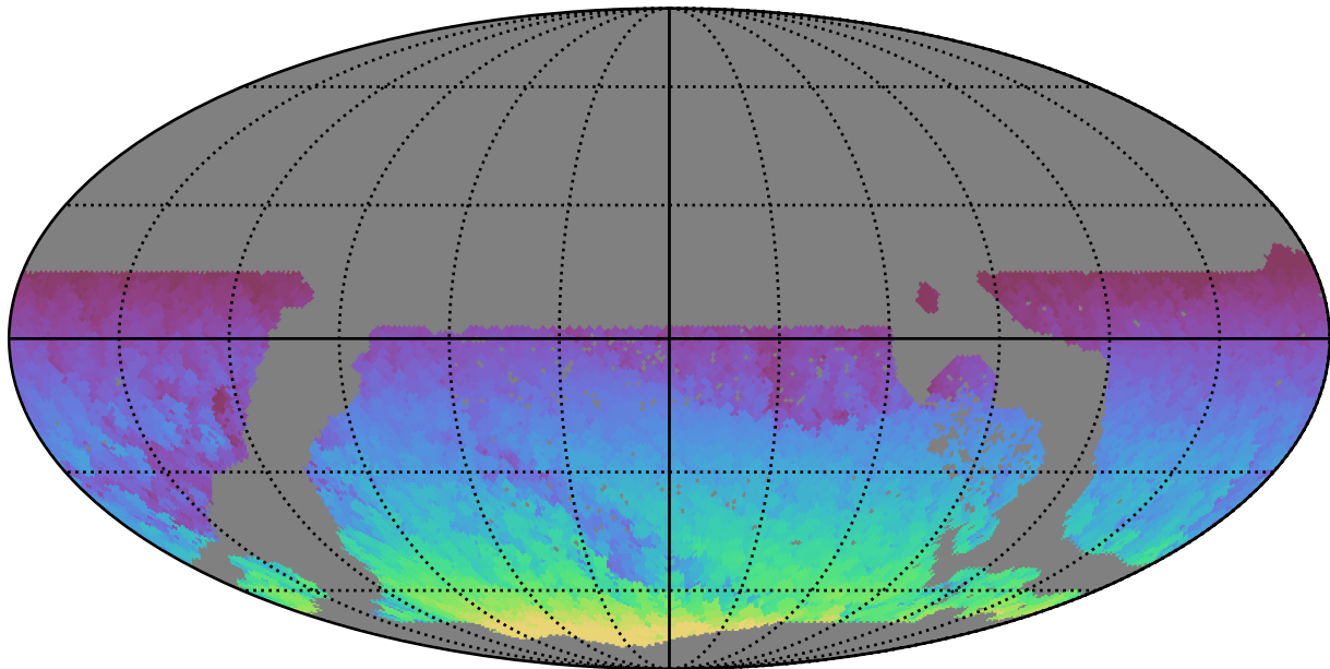
ddf_acor_sf10_lsf15_lsr20_v3.4_10yrs WFD all bands: Max HA
