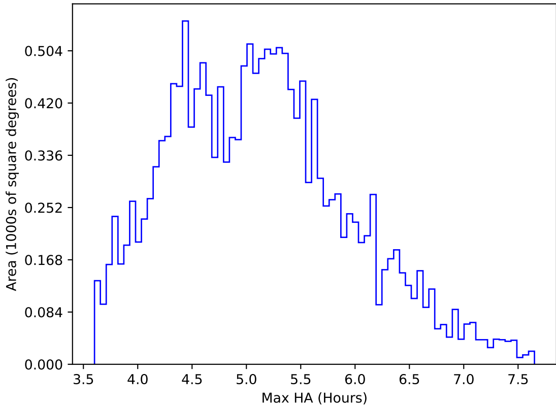
ddf_acor_sf10_lsf15_lsr20_v3.4_10yrs WFD all bands: Max HA
