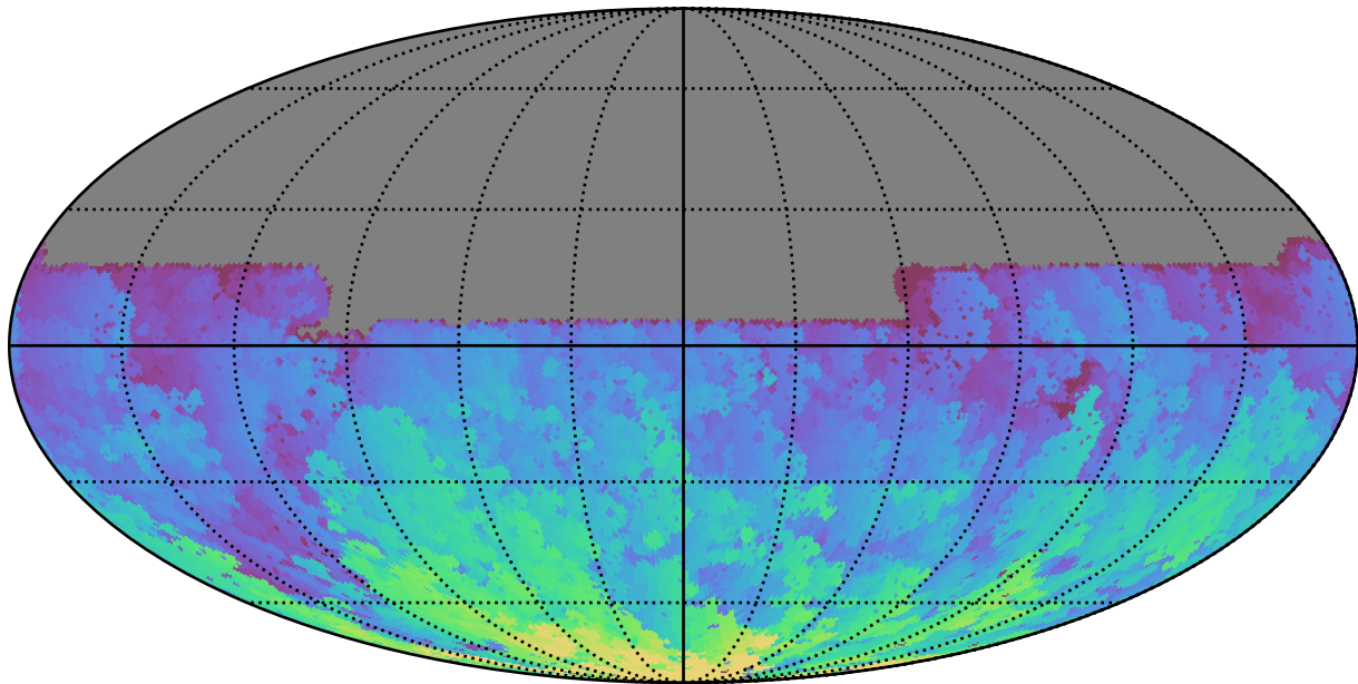
ddf_acor_sf10_lsf15_lsr20_v3.4_10yrs All sky u band: Max HA
