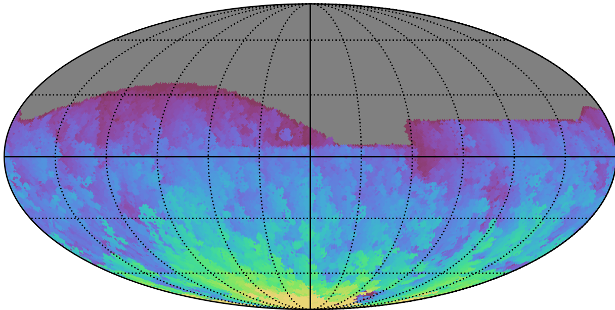
ddf_acor_sf10_lsf15_lsr20_v3.4_10yrs All sky r band: Max HA
