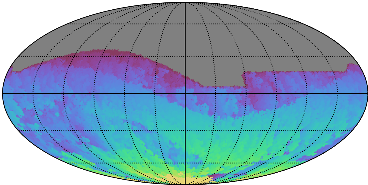
ddf_acor_sf10_lsf15_lsr20_v3.4_10yrs All sky i band: Max HA
