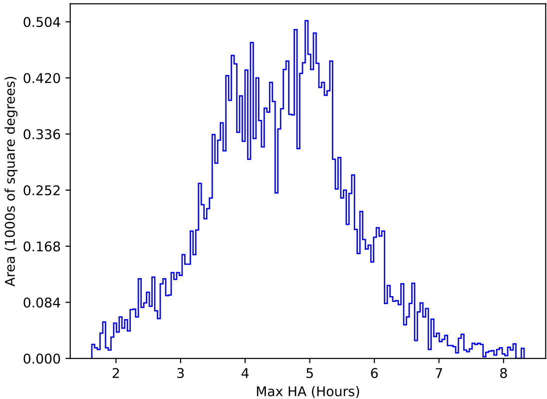
ddf_acor_sf10_ls15_lsr20_v3.4_10yrs All sky i band: Max HA
