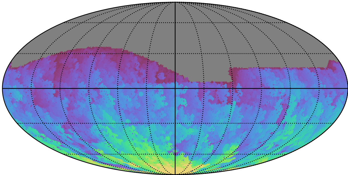
ddf_acor_sf10_lsf15_lsr20_v3.4_10yrs All sky g band: Max HA
