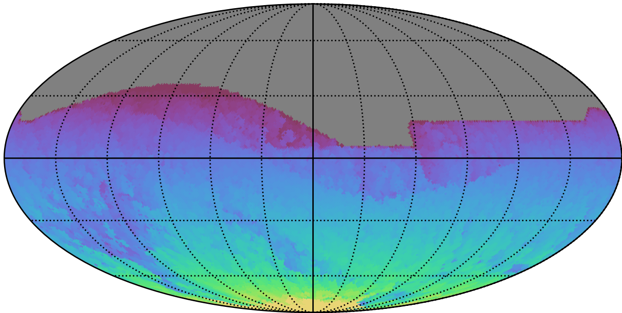
ddf_acor_sf10_lsf15_lsr20_v3.4_10yrs All sky all bands: Max HA
