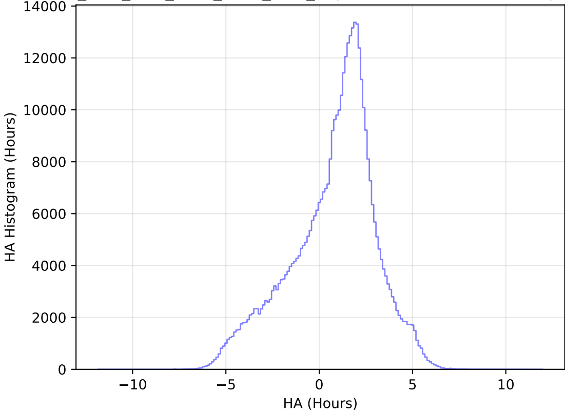
ddf_acor_sf10_ls15_lsr20_v3.4_10yrs WFD z band: HA Histogram
