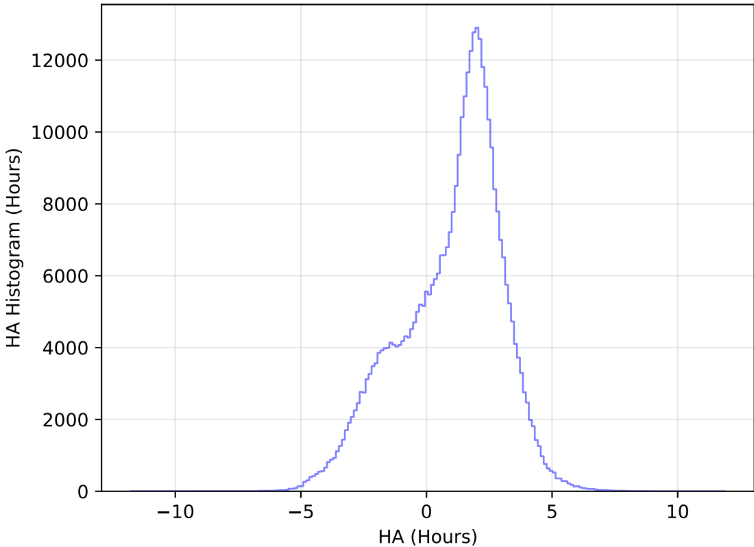
ddf_acor_sf10_lsf15_lsr20_v3.4_10yrs WFD y band: HA Histogram
