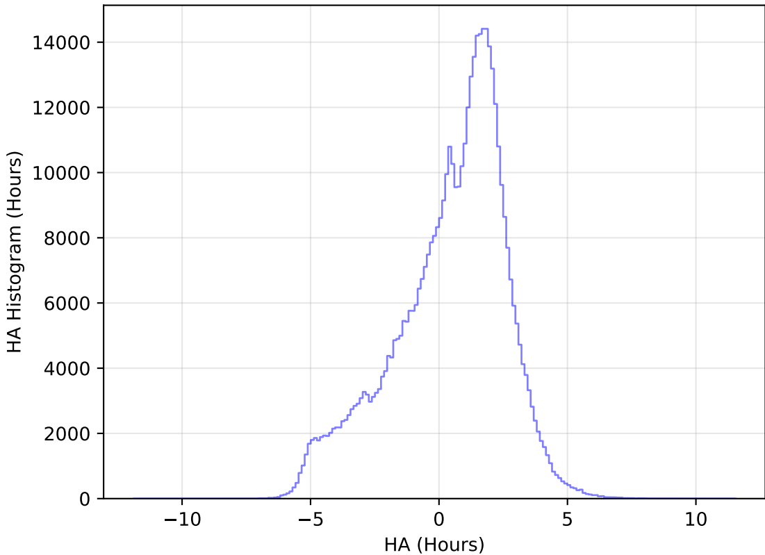
ddf_acor_sf10_lsf15_lsr20_v3.4_10yrs WFD r band: HA Histogram
