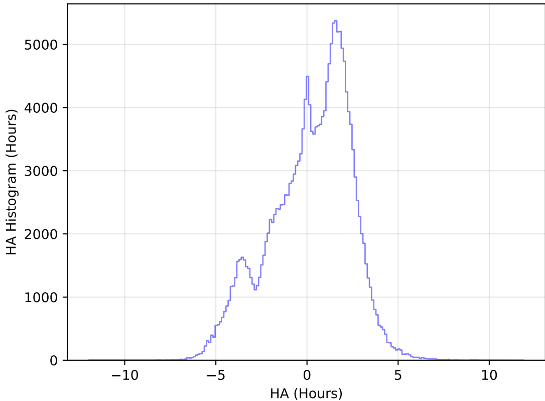
ddf_acor_sf10_lsf15_lsr20_v3.4_10yrs WFD g band: HA Histogram
