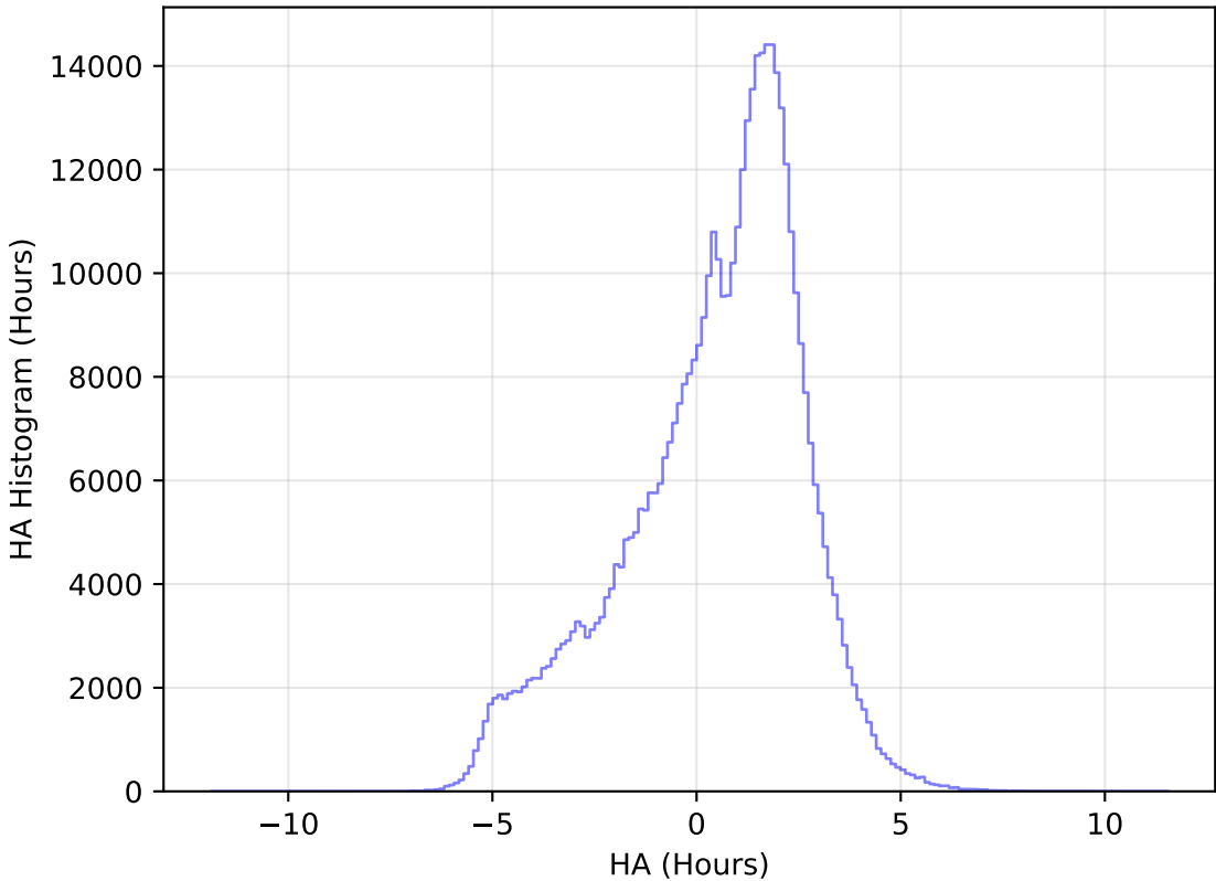
ddf_acor_sf10_lsf15_lsr20_v3.4_10yrs All sky r band: HA Histogram
