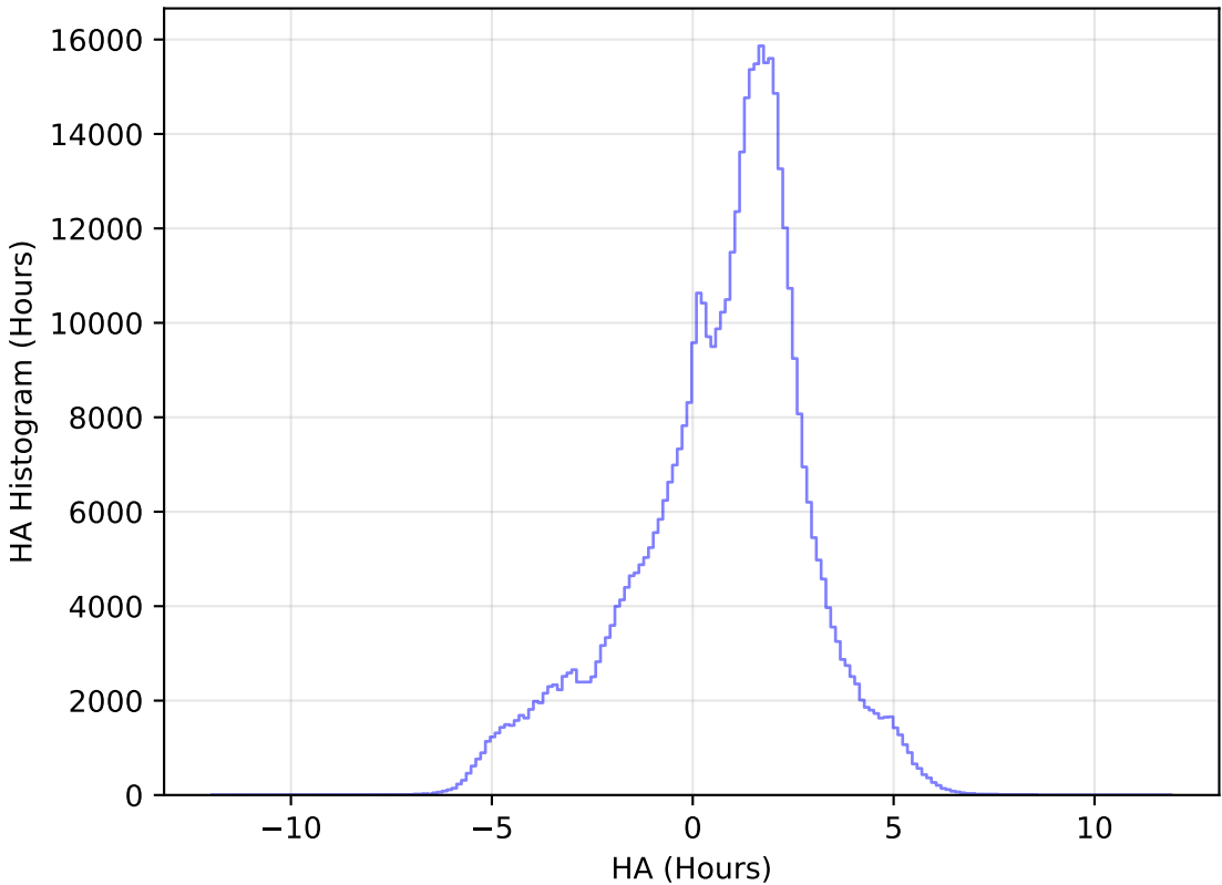
ddf_acor_sf10_lsf15_lsr20_v3.4_10yrs All sky i band: HA Histogram
