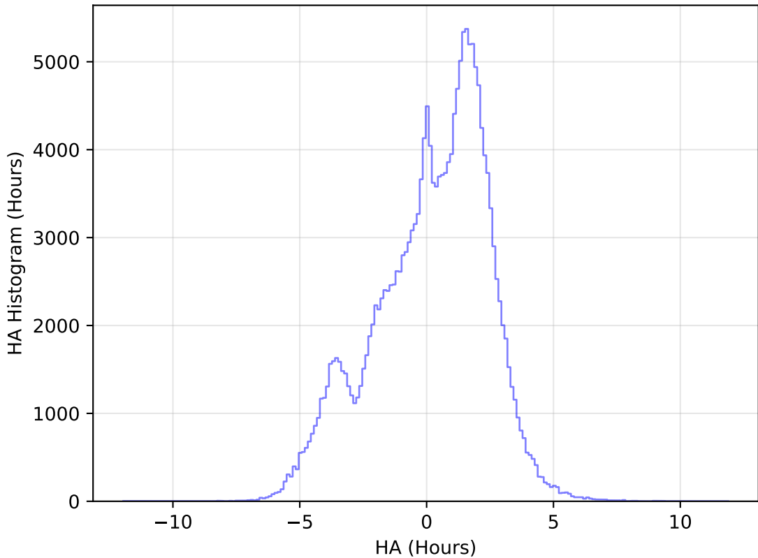
ddf_acor_sf10_lsf15_lsr20_v3.4_10yrs All sky g band: HA Histogram
