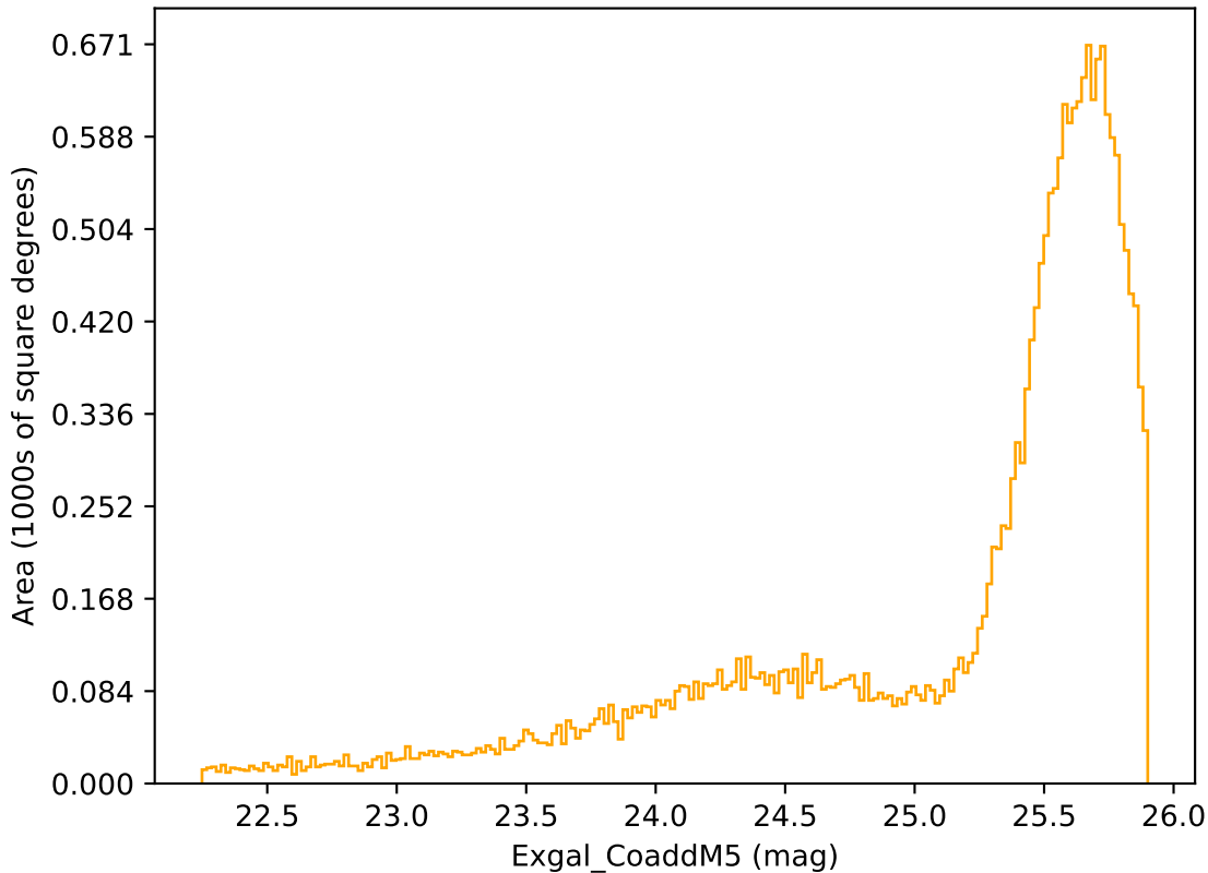
ddf_acor_sf10_lsf15_lsr20_v3.4_10yrs Yr 1 r band: Exgal_CoaddM5
