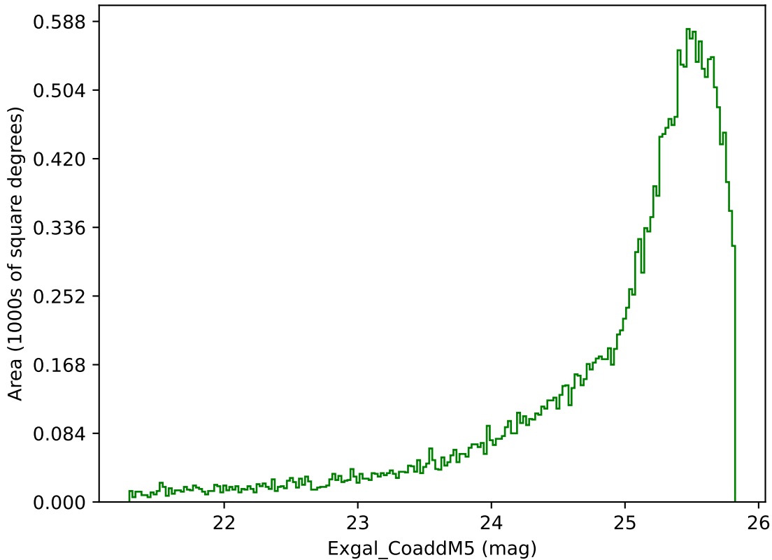
ddf_acor_sf10_lsf15_lsr20_v3.4_10yrs Yr 1 g band: Exgal_CoaddM5
