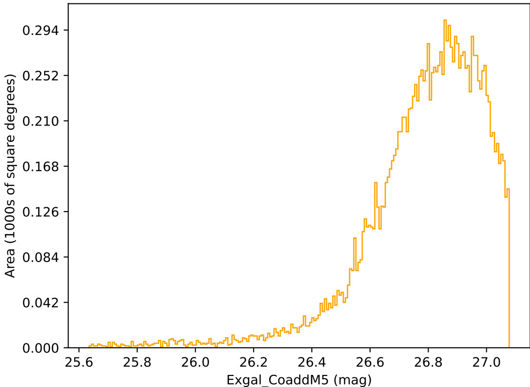
ddf_acor_sf10_lsf15_lsr20_v3.4_10yrs WFD r band: Exgal_CoaddM5
