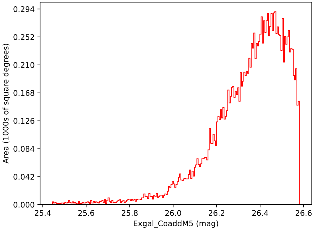
ddf_acor_sf10_lsf15_lsr20_v3.4_10yrs WFD i band: Exgal_CoaddM5
