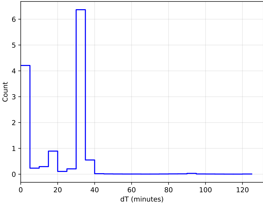
ddf_acor_sf10_lsf15_lsr20_v3.4_10yrs All sky: DeltaT Histogram
