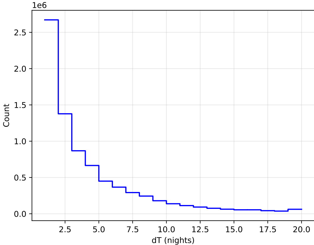
ddf_acor_sf10_lsf15_lsr20_v3.4_10yrs WFD all bands: DeltaNight Histogram
