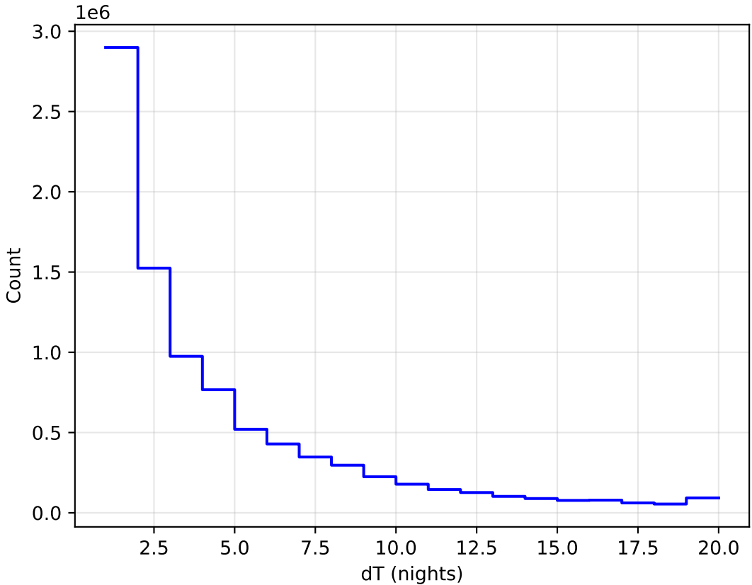
ddf_acor_sf10_lsf15_lsr20_v3.4_10yrs All sky all bands: DeltaNight Histogram
