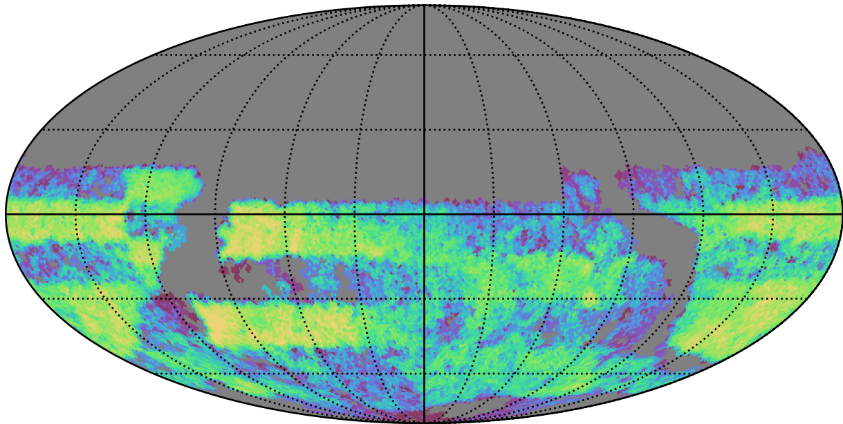
ddf_acor_sf10_lsf15_lsr20_v3.4_10yrs Yr 3-4 u band: CoaddM5
