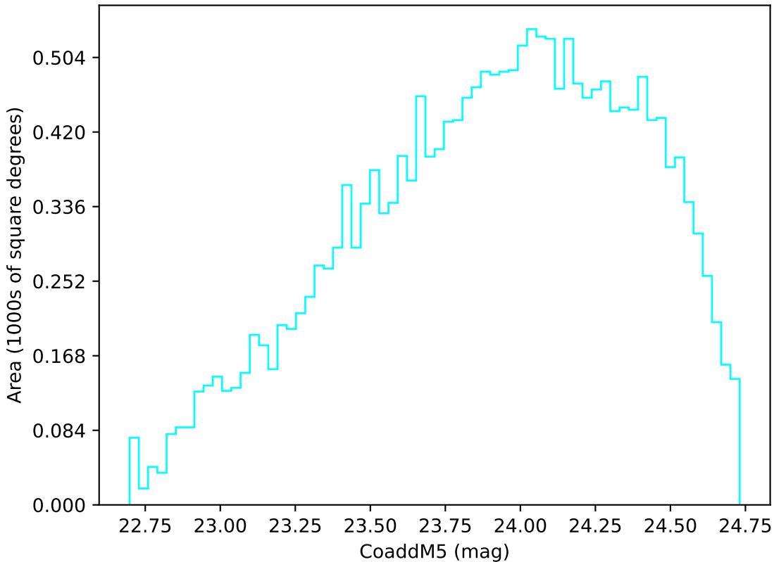
ddf_acor_sf10_lsf15_lsr20_v3.4_10yrs Yr 3-4 u band: CoaddM5
