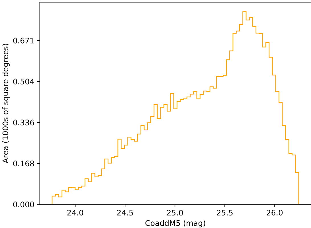
ddf_acor_sf10_lsf15_lsr20_v3.4_10yrs Yr 3-4 r band: CoaddM5
