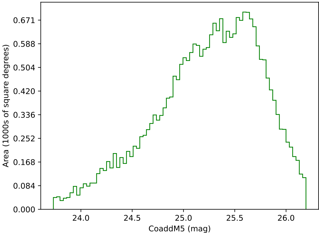
ddf_acor_sf10_lsf15_lsr20_v3.4_10yrs Yr 3-4 g band: CoaddM5
