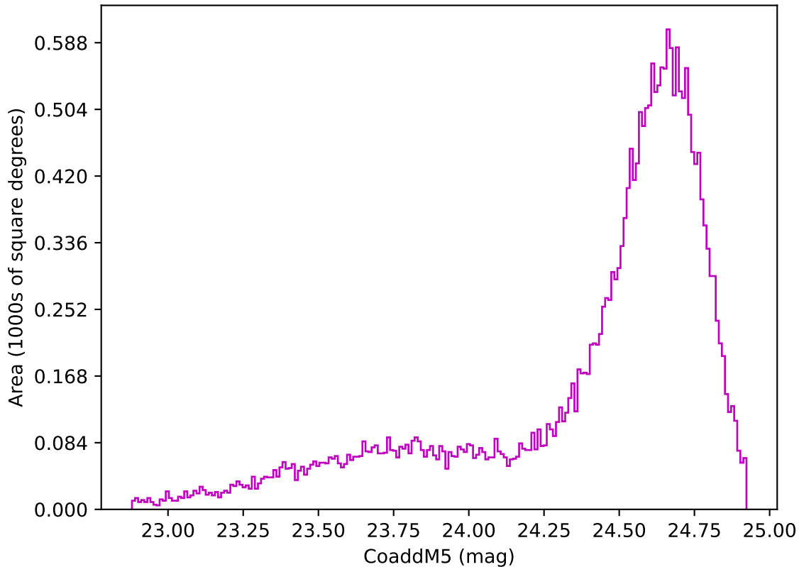
ddf_acor_sf10_ls15_lsr20_v3.4_10yrs Yr 1 z band: CoaddM5
