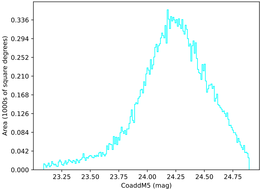
ddf_acor_sf10_lsf15_lsr20_v3.4_10yrs Yr 1 u band: CoaddM5
