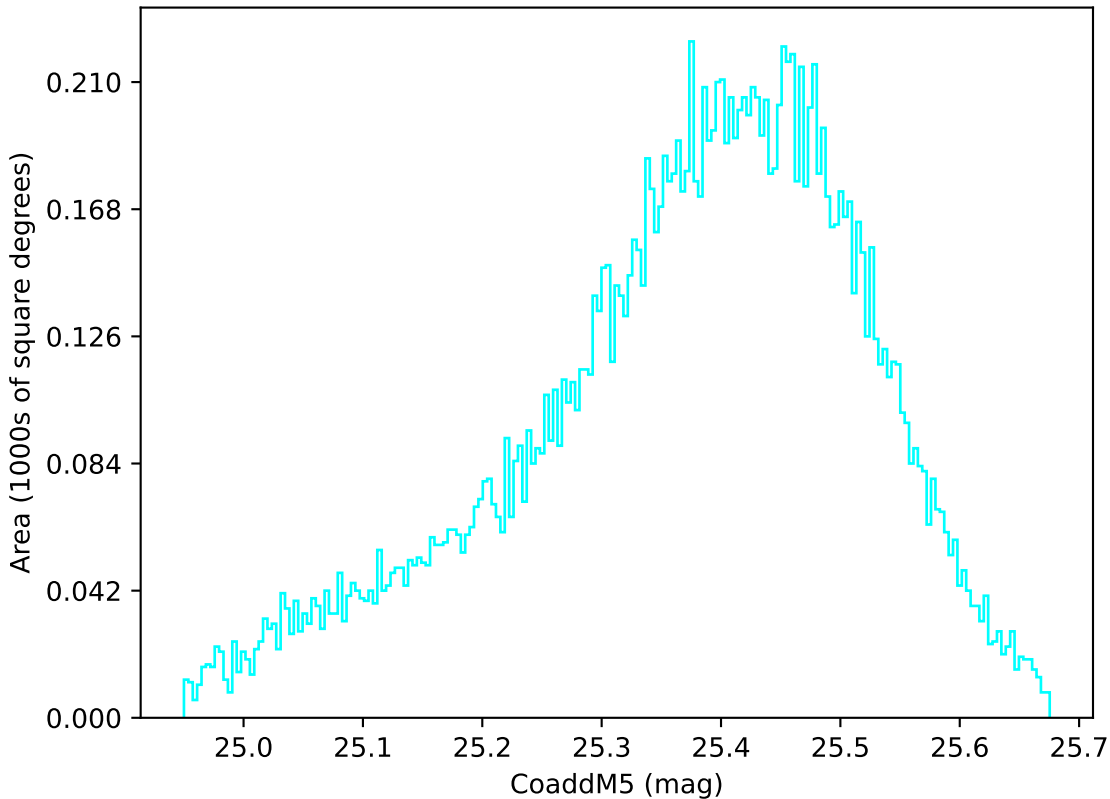
ddf_acor_sf10_lsf15_lsr20_v3.4_10yrs WFD u band: CoaddM5
