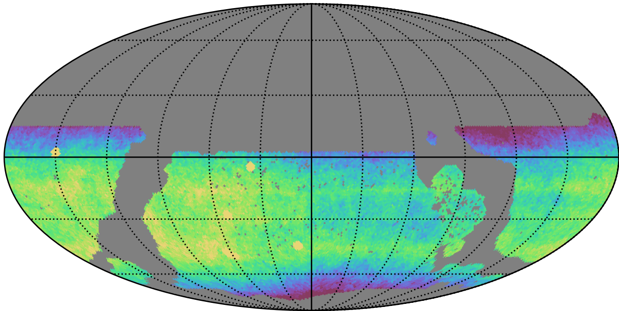
ddf_acor_sf10_lsf15_lsr20_v3.4_10yrs WFD i band: CoaddM5
