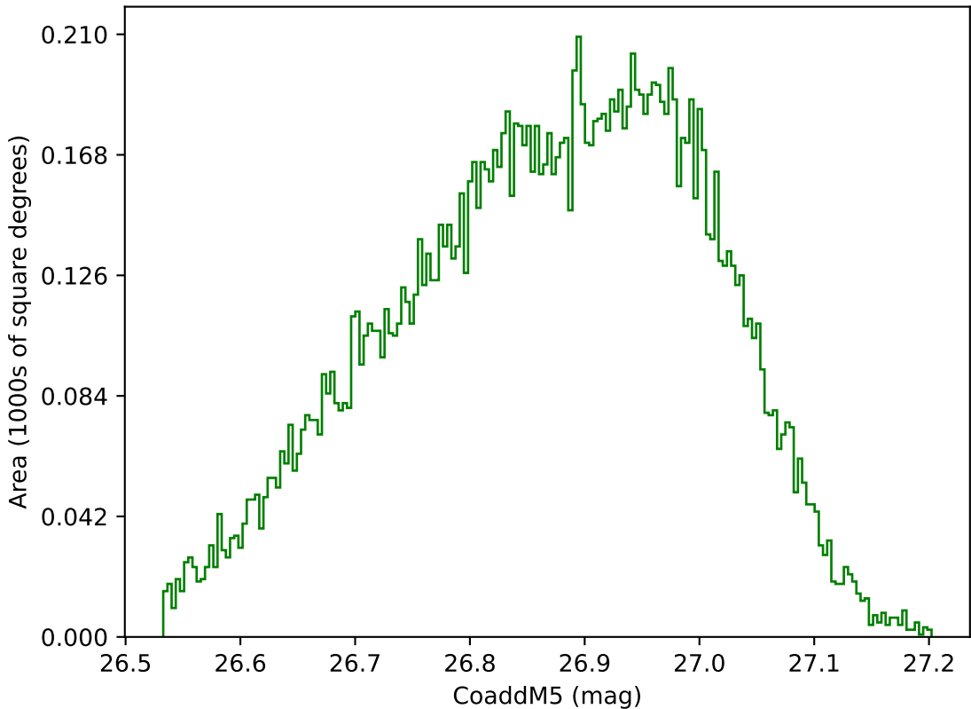
ddf_acor_sf10_lsf15_lsr20_v3.4_10yrs WFD g band: CoaddM5
