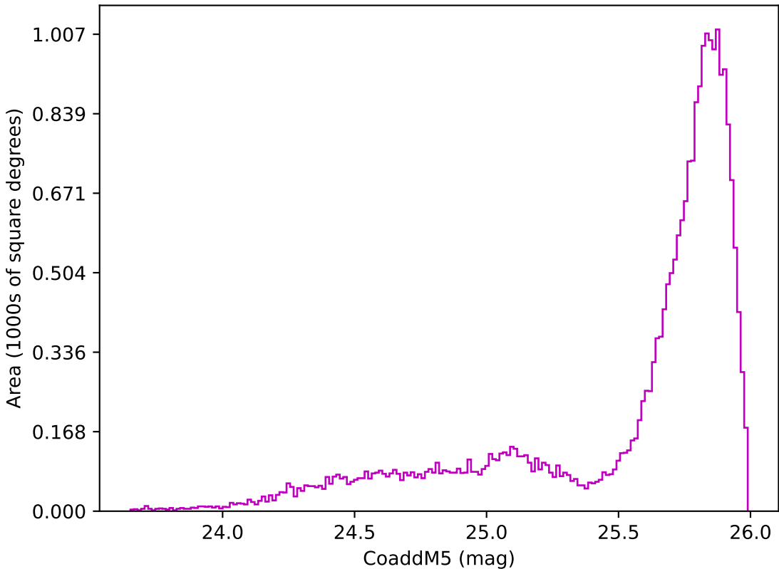
ddf_acor_sf10_lsf15_lsr20_v3.4_10yrs All sky z band: CoaddM5
