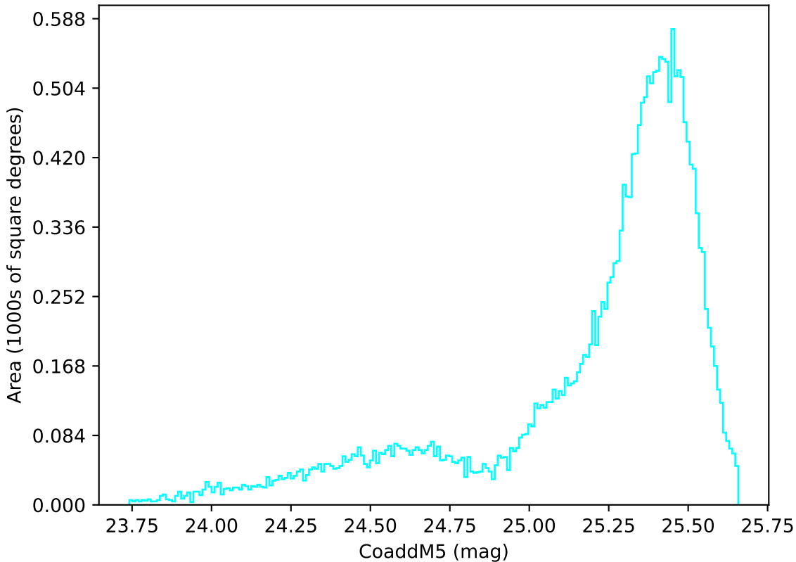
ddf_acor_sf10_lsf15_lsr20_v3.4_10yrs All sky u band: CoaddM5
