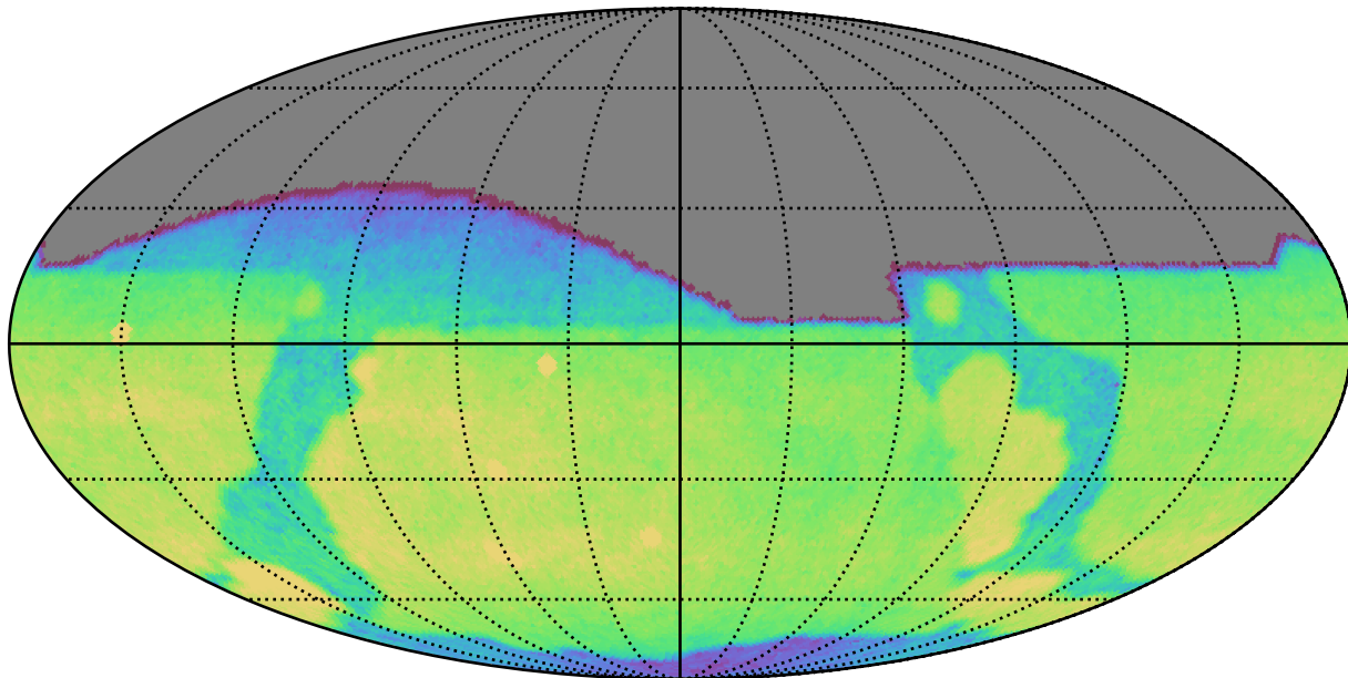
ddf_acor_sf10_lsf15_lsr20_v3.4_10yrs All sky g band: CoaddM5
