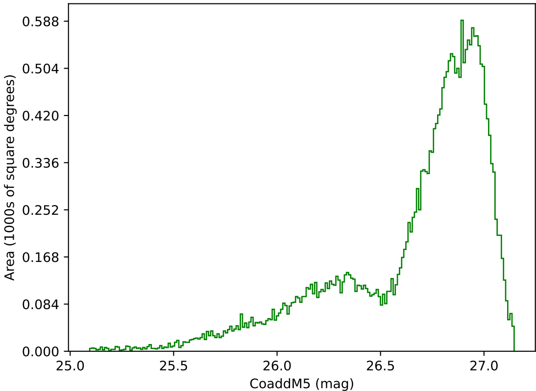
ddf_acor_sf10_lsf15_lsr20_v3.4_10yrs All sky g band: CoaddM5
