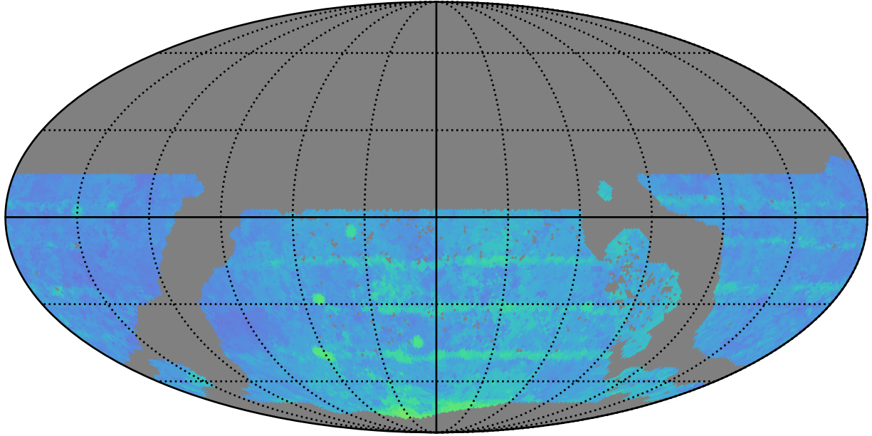
ddf_acor_sf10_lsf15_lsr20_v3.4_10yrs WFD z band: 80thPercentile Season Length
